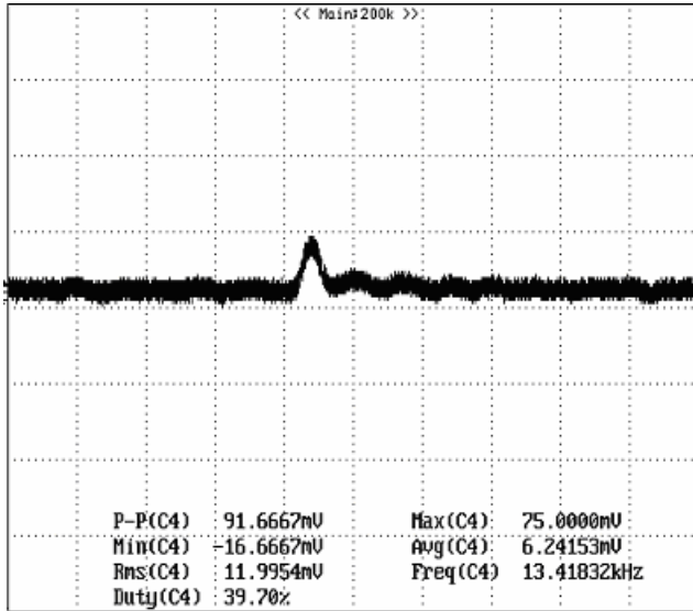
Figure 9: Output voltage response to step-change in load current (75%-50% of I_o , max; di/dt = 0.1A/\mu s ). Load cap: 10\mu F , tantalum capacitor and 1\mu F ceramic capacitor. Trace: V_{out} (50mV/div, 100us/div). Scope measurement should be made using a BNC cable (length shorter than 20 inches). Position the load between 51 mm to 76 mm (2 inches to 3 inches) from the module..
