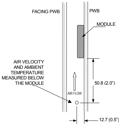
Figure 21: Wind tunnel test setup
