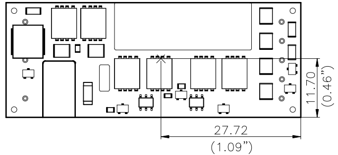
Figure 22: Hot spot location. Pin locations are for reference only. *The allowed maximum hot spot temperature is defined at 123°C
