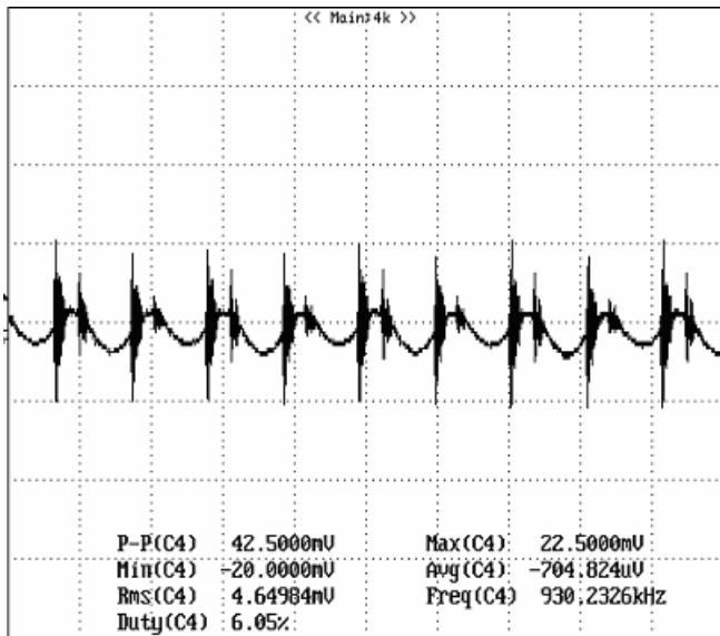
Figure 15: Output voltage ripple at nominal input voltage and rated load current ( I_o=10\text{A} ) (20 mV/div, 2us/div) Load capacitance: 1\mu\text{F} ceramic capacitor and 10\mu\text{F} tantalum capacitor. Bandwidth: 20 MHz. Scope measurements should be made using a BNC cable (length shorter than 20 inches). Position the load between 51 mm to 76 mm (2 inches to 3 inches) from the module.
