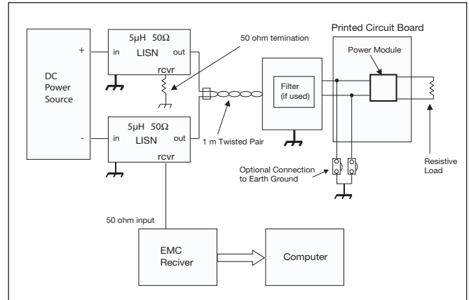
Test set-up.
