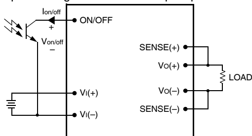
Figure 34. Remote On/Off Implementation.
