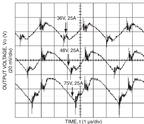
Figure 3. Output Ripple Voltage ( I_O = I_{O, \text{max}} ). Tyco Electronics Power Systems
