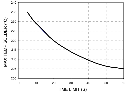
Figure 55. Time Limit Curve Above 205°C Reflow .
