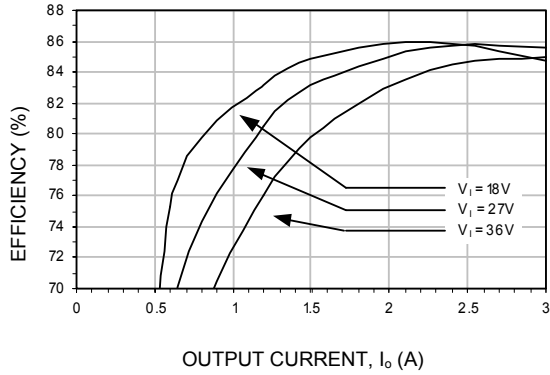
Figure 31. Converter Efficiency Vs Load.
