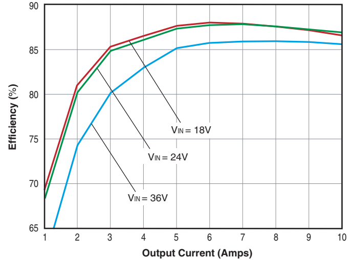
UHE-1.8/10000-D48 Efficiency vs. Load @ +25°C Ambient
